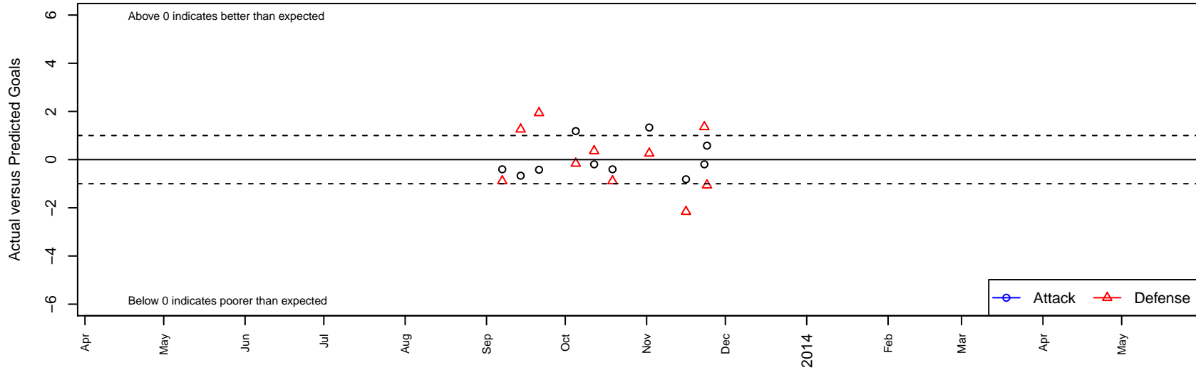
Juventus SC Bianco B99 Dots are actual minus expected GF (blue circles) and GA (red triangles). Blue line is smoothed change in attack strength. Red is smoothed change in defense strength.
